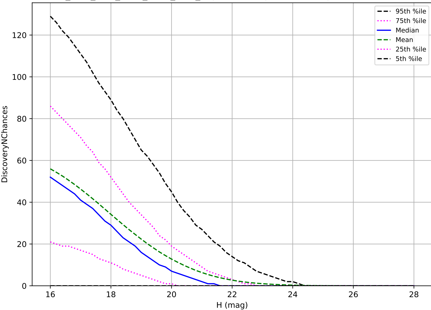
ddf_acor_sf25_lsf30_lsr10_v3.4_10yrs: NEO 3 pairs in 15 nights detection loss
