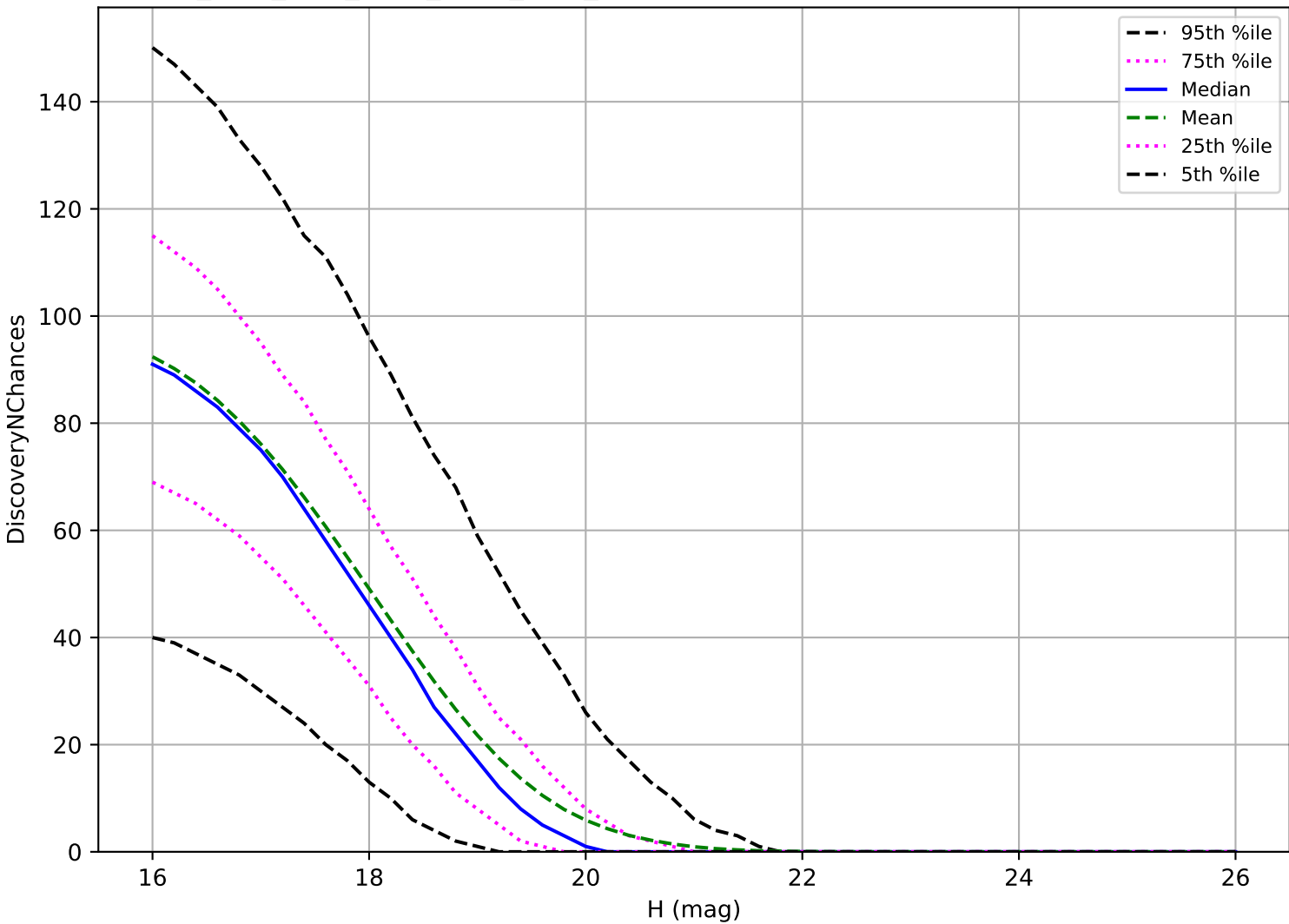
ddf_acor_sf25_lsf30_lsr10_v3.4_10yrs: MBA 3 pairs in 15 nights detection loss
