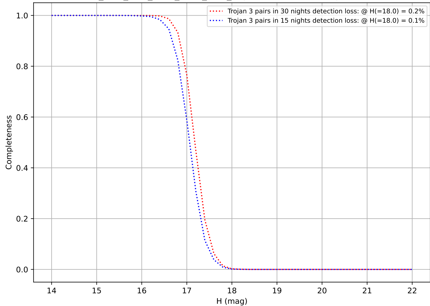
ddf_acor_sf25_lsf30_lsr10_v3.4_10yrs: DifferentialCompleteness
