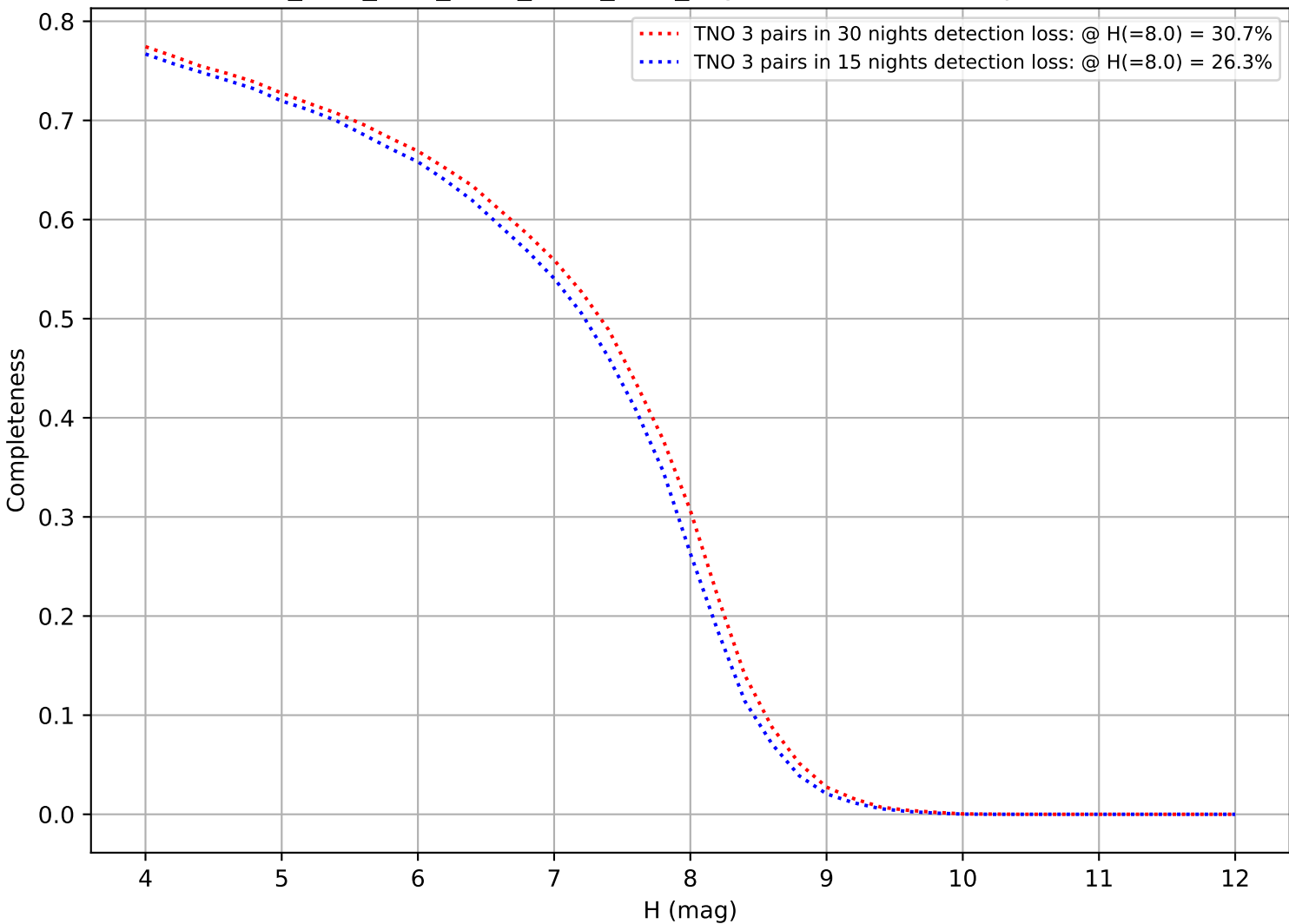
ddf_acor_sf25_lsf30_lsr10_v3.4_10yrs: DifferentialCompleteness
