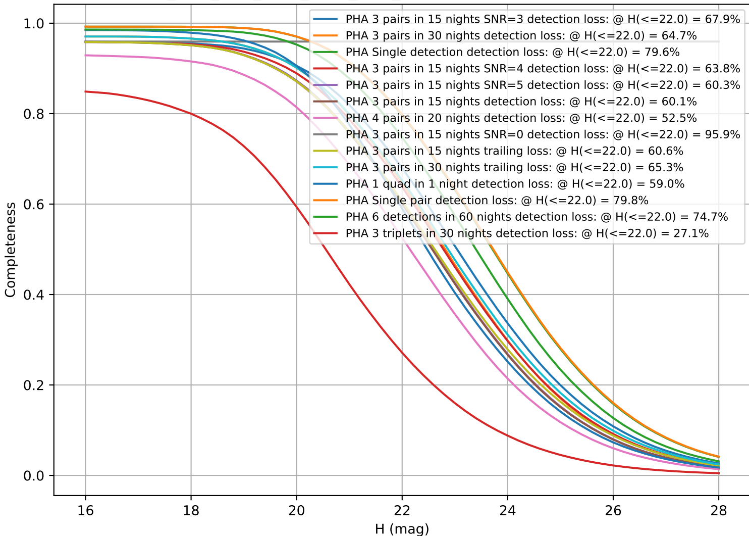
ddf_acor_sf25_lsf30_lsr10_v3.4_10yrs: CumulativeCompleteness
