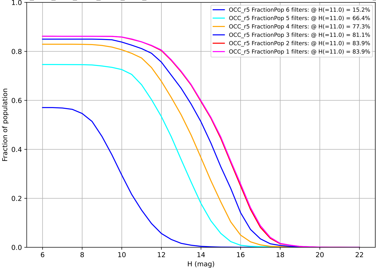
ddf_acor_sf25_lsf30_lsr10_v3.4_10yrs: Fraction of population with colors in X filters OCC_r5
