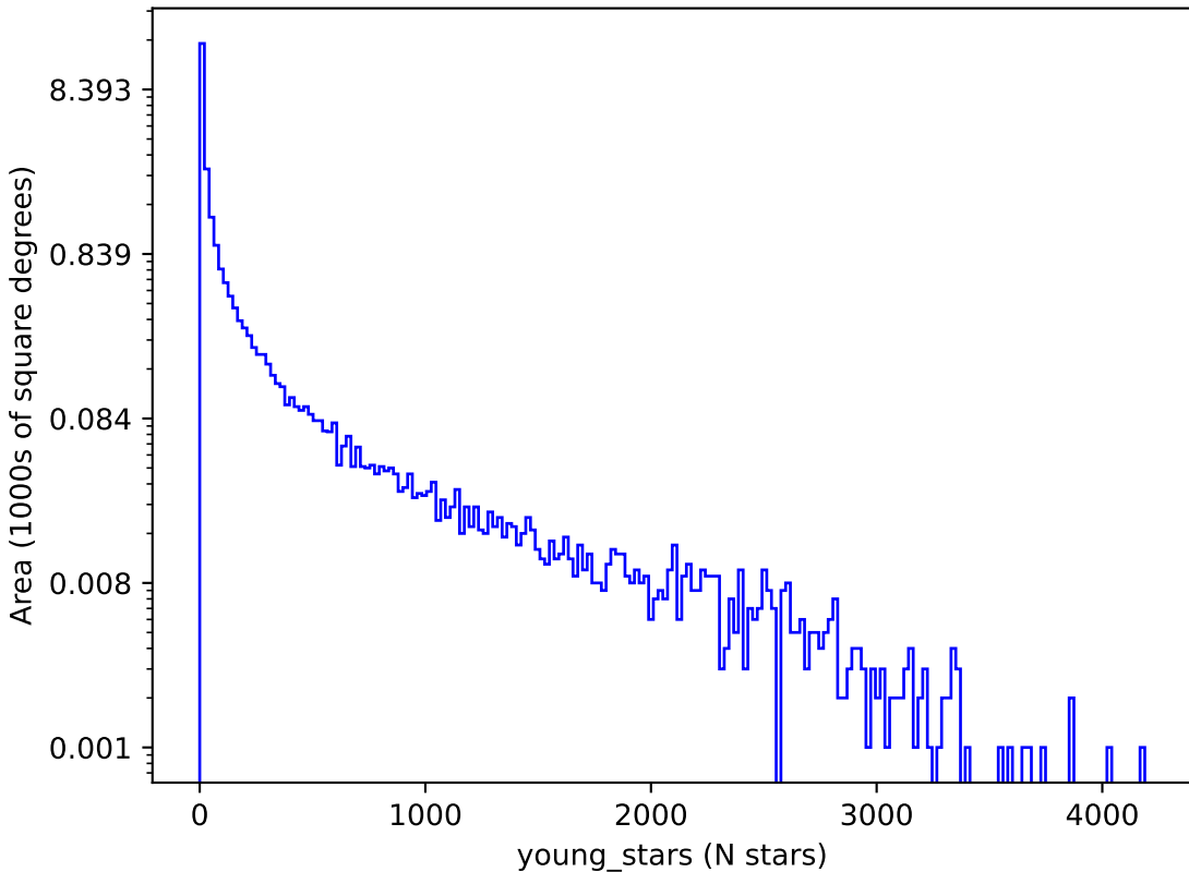
ddf_acor_sf25_lsf30_lsr10_v3.4_10yrs : young_stars
