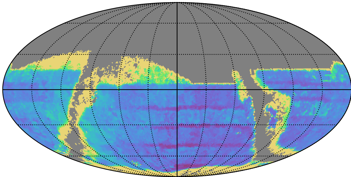
ddf_acor_sf25_lsf30_lsr10_v3.4_10yrs : TDC_accuracy
