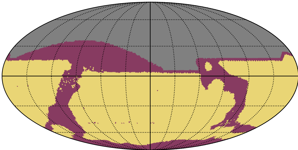
ddf_acor_sf25_lsf30_lsr10_v3.4_10yrs : RapidRevisits
