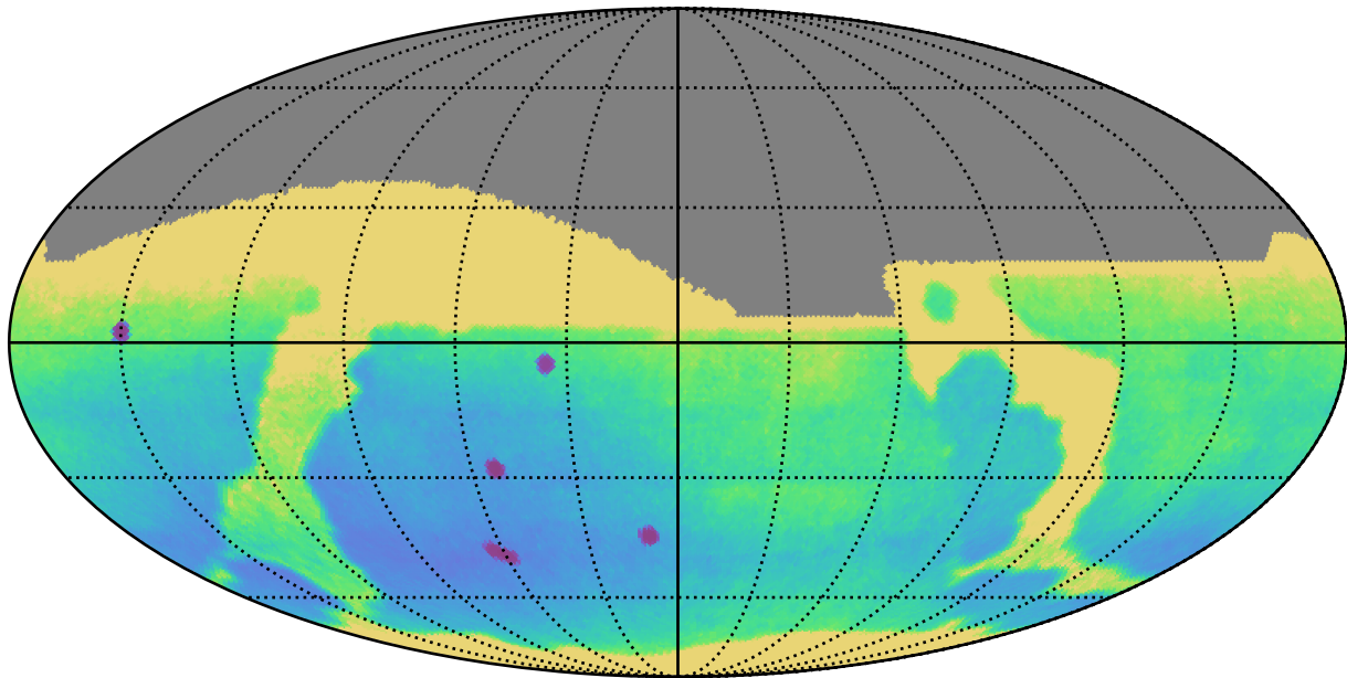
ddf_acor_sf25_lsf30_lsr10_v3.4_10yrs : Parallax Uncert @ 24.0
