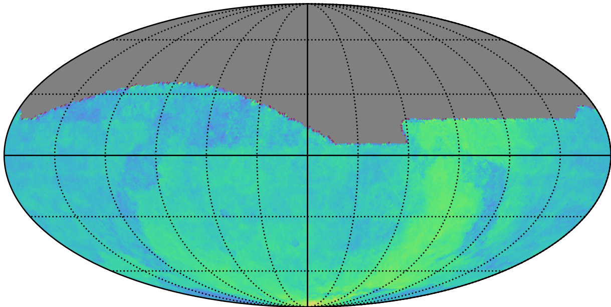
ddf_acor_sf25_lsf30_lsr10_v3.4_10yrs : Parallax Coverage @ 24.0
