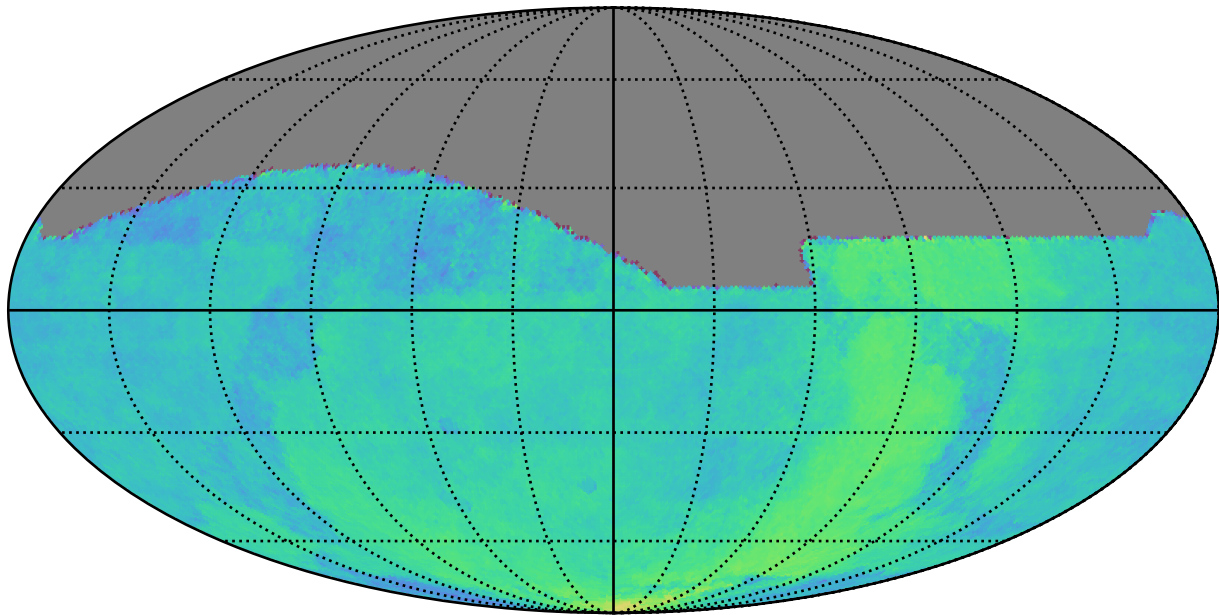
ddf_acor_sf25_lsf30_lsr10_v3.4_10yrs : Parallax Coverage @ 22.4
