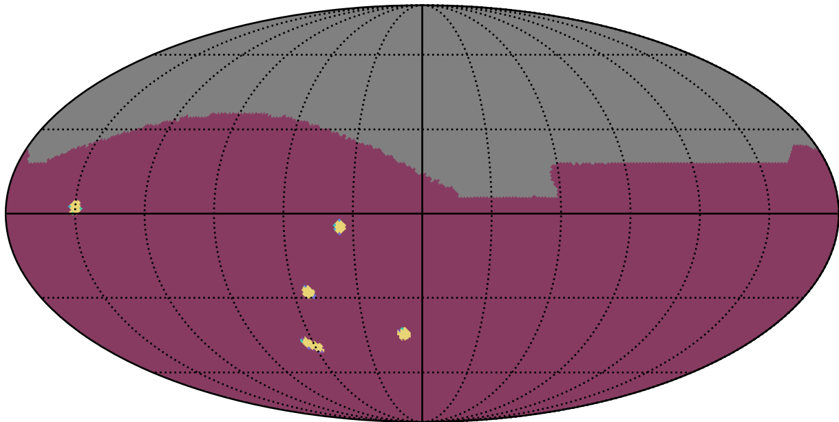
ddf_acor_sf25_lsf30_lsr10_v3.4_10yrs : NumberOfQuickRevisits
