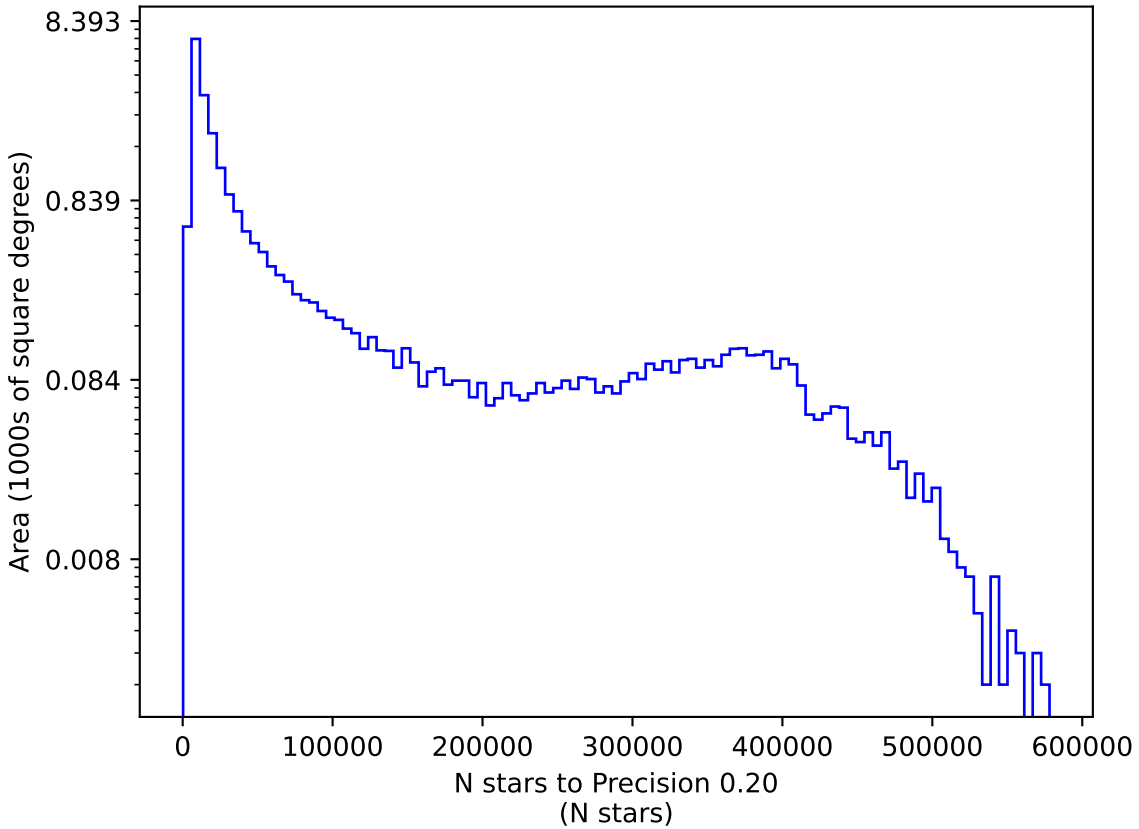
ddf_acor_sf25_lsf30_lsr10_v3.4_10yrs y: N stars to Precision 0.20
