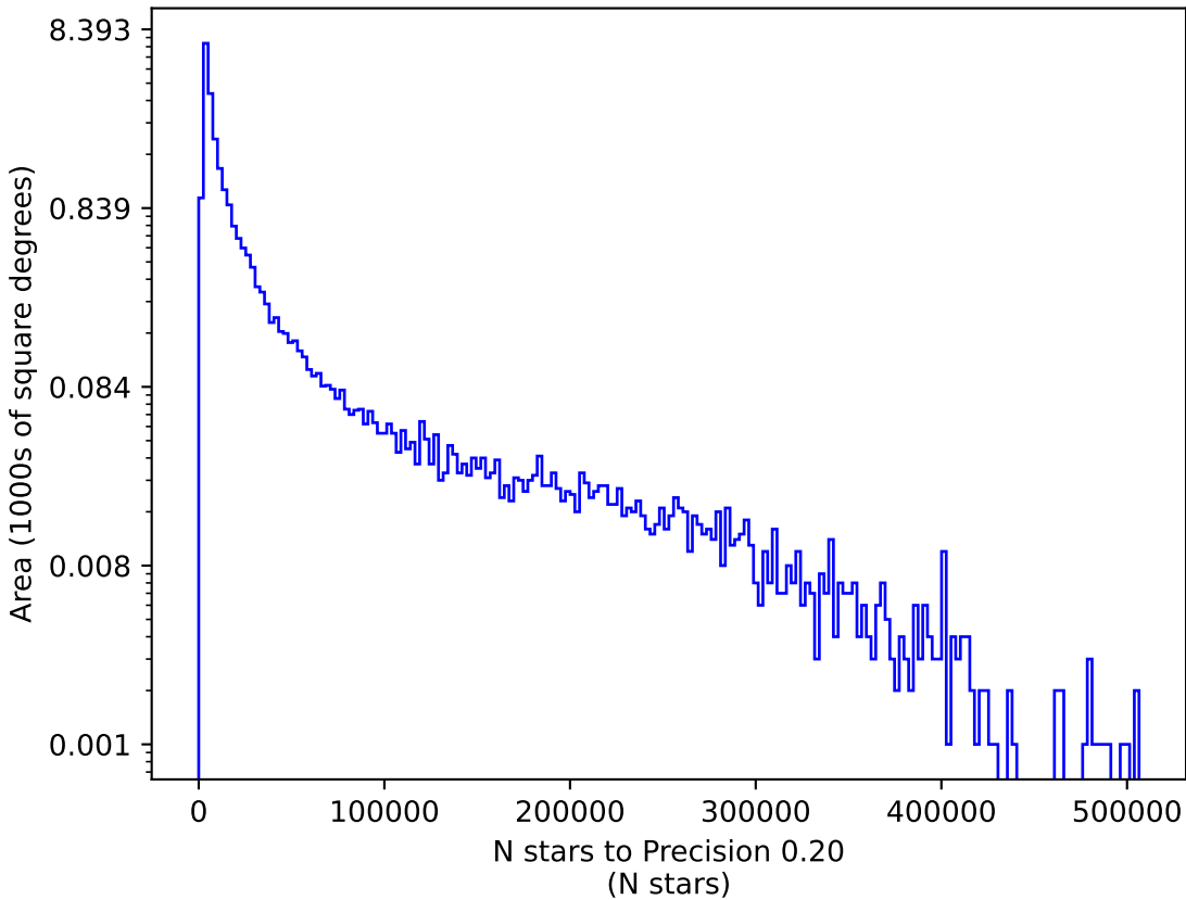
ddf_acor_sf25_ls30_lsr10_v3.4_10yrs u: N stars to Precision 0.20
