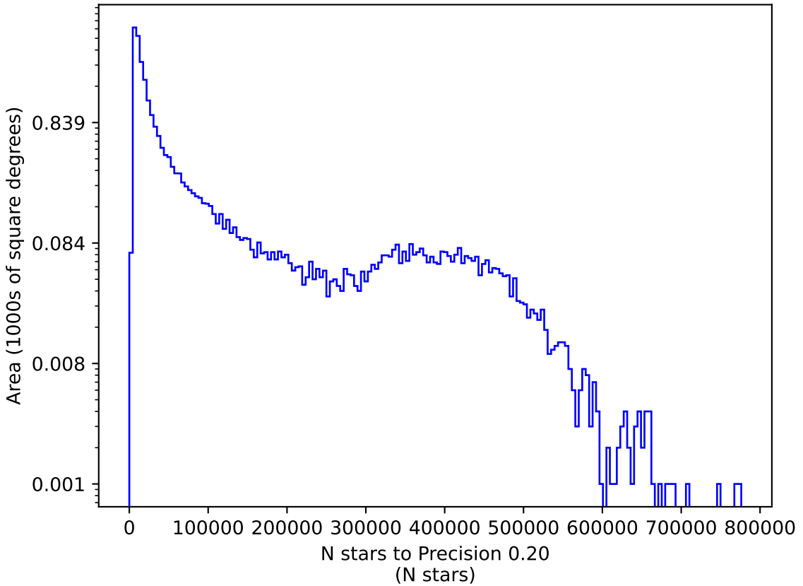
ddf_acor_sf25_lsf30_lsr10_v3.4_10yrs r: N stars to Precision 0.20
