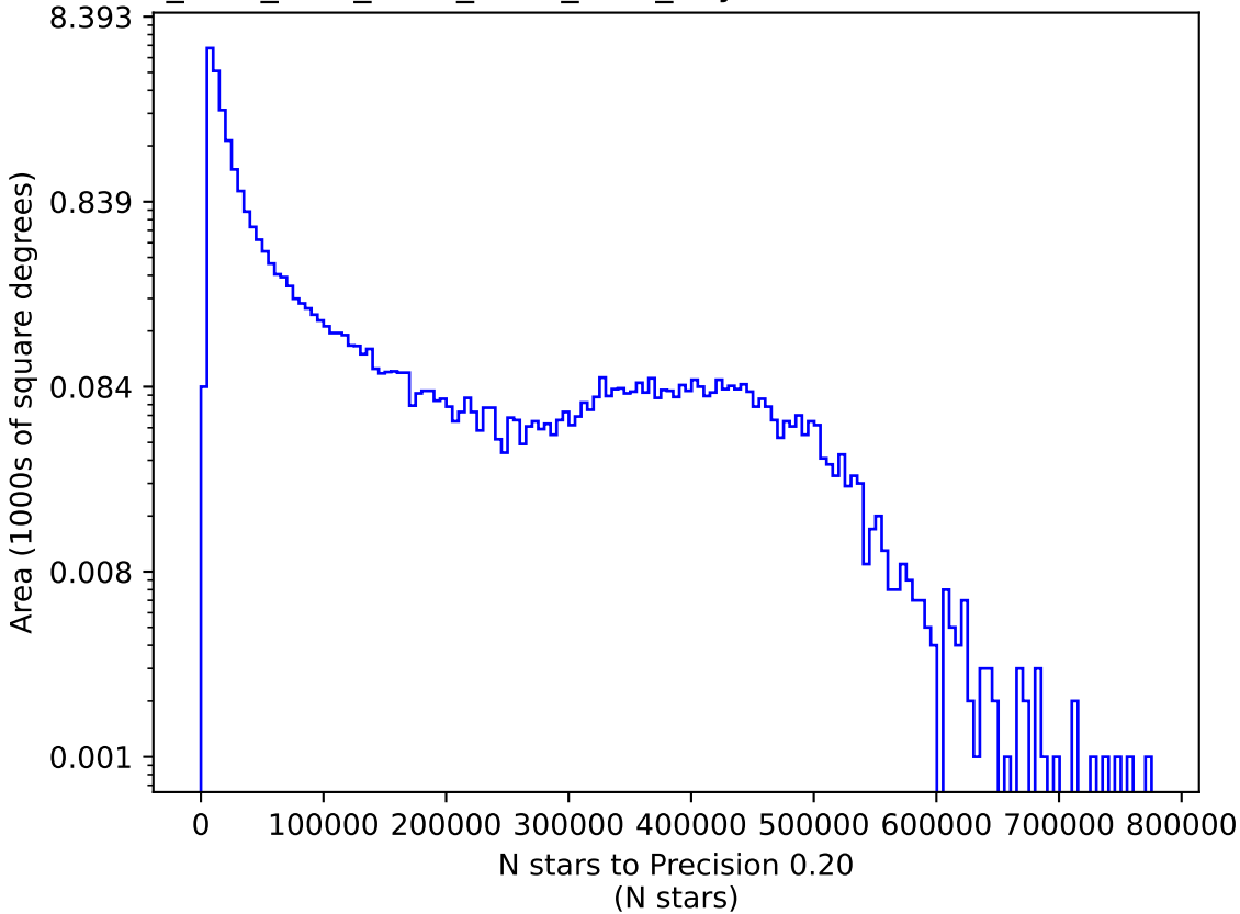
ddf_acor_sf25_lsf30_lsr10_v3.4_10yrs i: N stars to Precision 0.20
