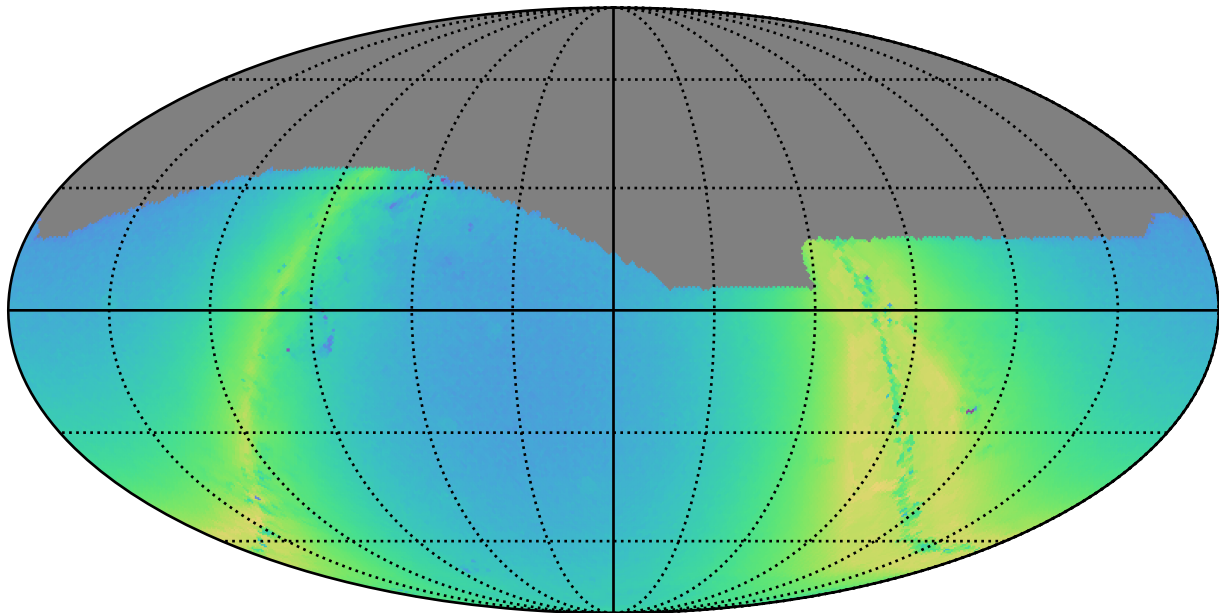
ddf_acor_sf25_lsf30_lsr10_v3.4_10yrs g: N stars to Precision 0.20
