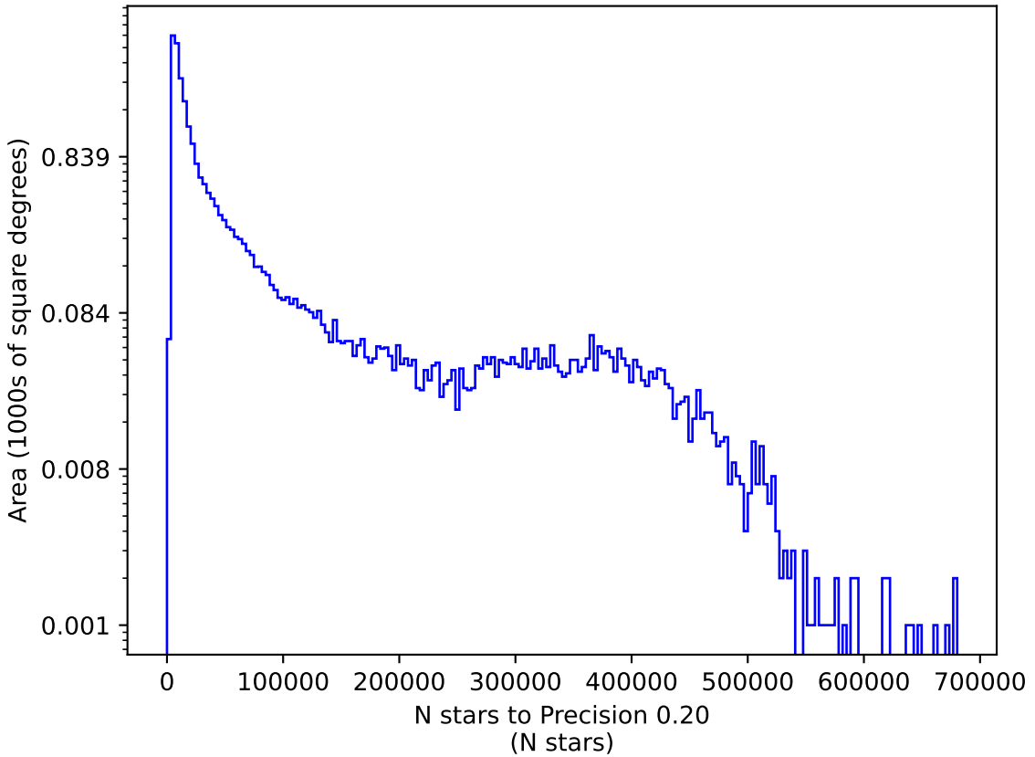
ddf_acor_sf25_lsf30_lsr10_v3.4_10yrs g: N stars to Precision 0.20
