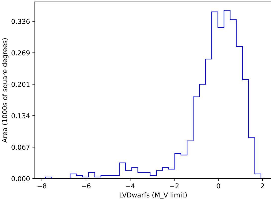
ddf_acor_sf25_lsf30_lsr10_v3.4_10yrs gi SCP: LVDwarfs
