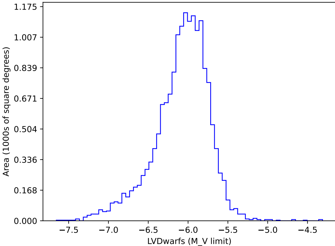
ddf_acor_sf25_lsf30_lsr10_v3.4_10yrs gi: LVDwarfs
