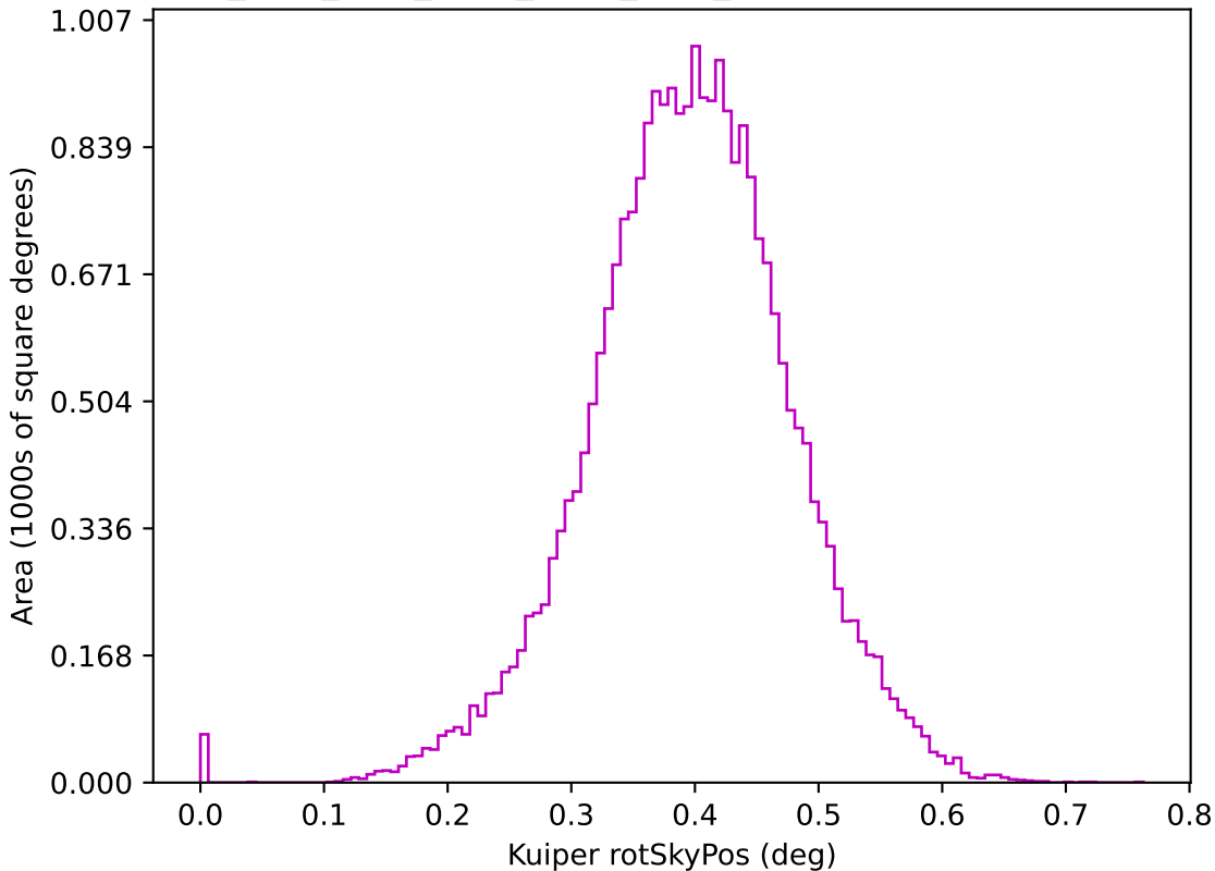
ddf_acor_sf25_ls30_lsr10_v3.4_10yrs z: Kuiper rotSkyPos
