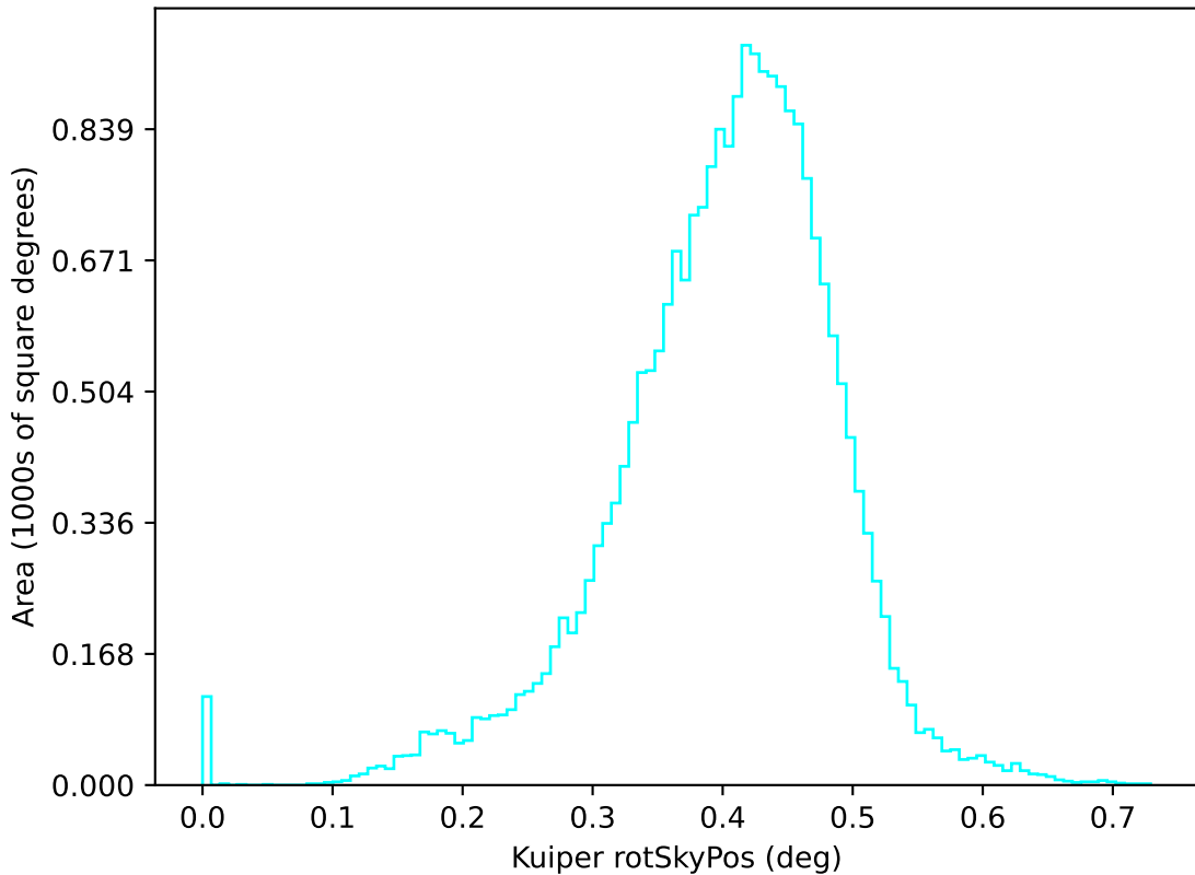
ddf_acor_sf25_lsf30_lsr10_v3.4_10yrs u: Kuiper rotSkyPos
