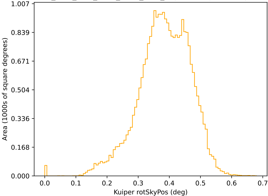
ddf_acor_sf25_lsf30_lsr10_v3.4_10yrs r: Kuiper rotSkyPos
