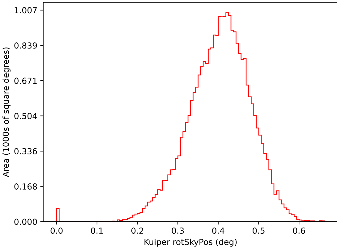
ddf_acor_sf25_ls30_lsr10_v3.4_10yrs i: Kuiper rotSkyPos
