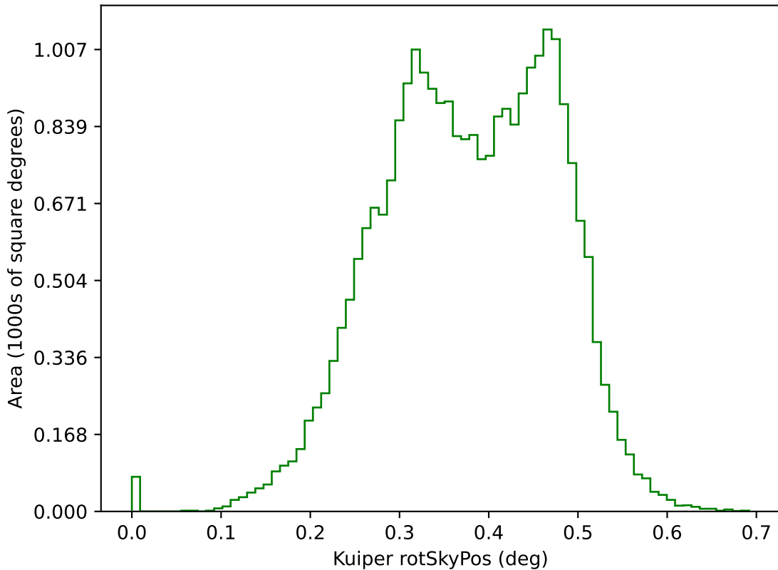
ddf_acor_sf25_lsf30_lsr10_v3.4_10yrs g: Kuiper rotSkyPos
