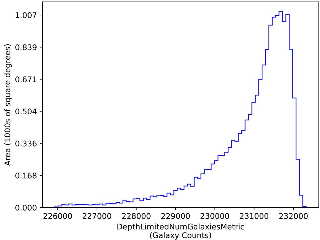
ddf_acor_sf25_lsf30_lsr10_v3.4_10yrs i band galaxies non-DD: DepthLimitedNumGalaxiesMetric
