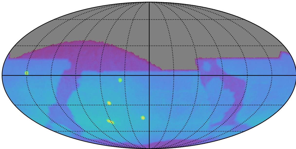
ddf_acor_sf25_lsf30_lsr10_v3.4_10yrs : Brown Dwarf, L7
