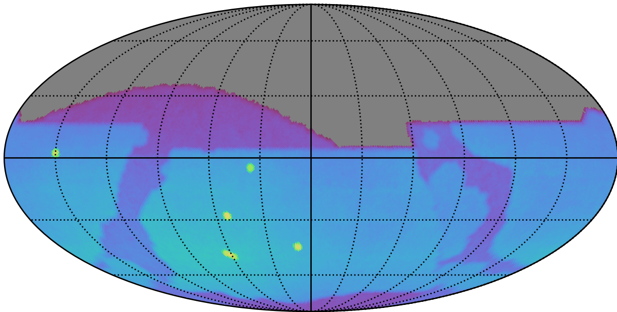
ddf_acor_sf25_lsf30_lsr10_v3.4_10yrs : Brown Dwarf, L4
