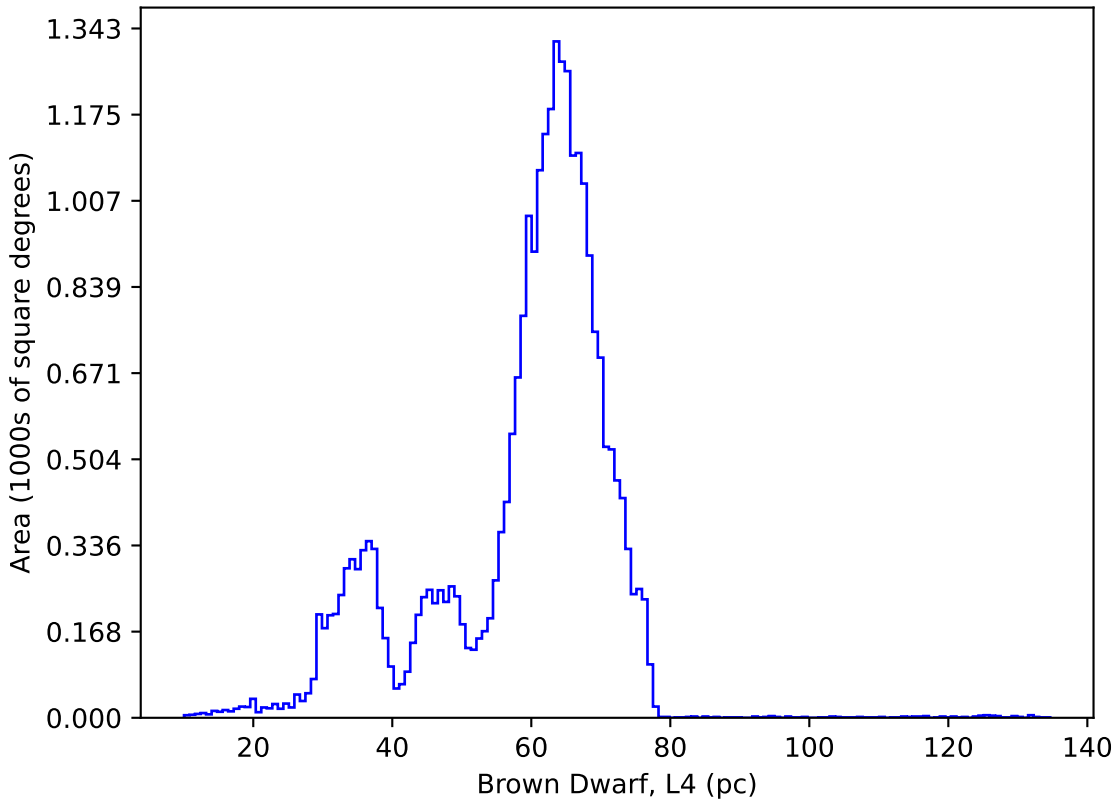
ddf_acor_sf25_lsf30_lsr10_v3.4_10yrs : Brown Dwarf, L4
