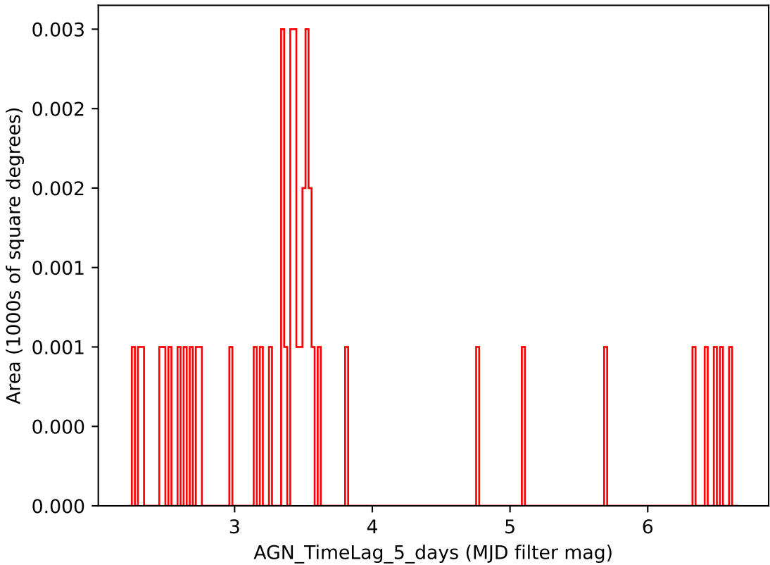
ddf_acor_sf25_ls30_lsr10_v3.4_10yrs i band: AGN_TimeLag_5_days
