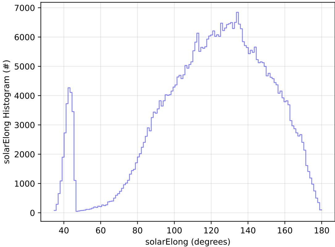
ddf_acor_sf25_lsf30_lsr10_v3.4_10yrs WFD z band: solarElong Histogram
