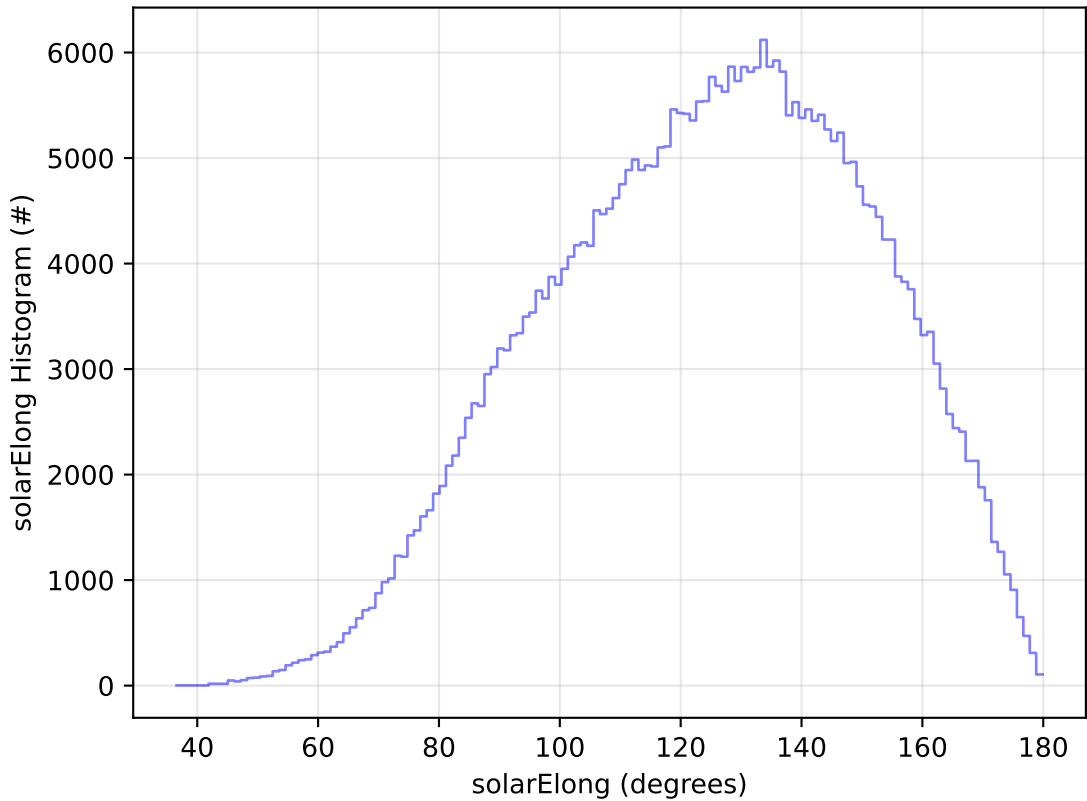
ddf_acor_sf25_lsf30_lsr10_v3.4_10yrs WFD y band: solarElong Histogram
