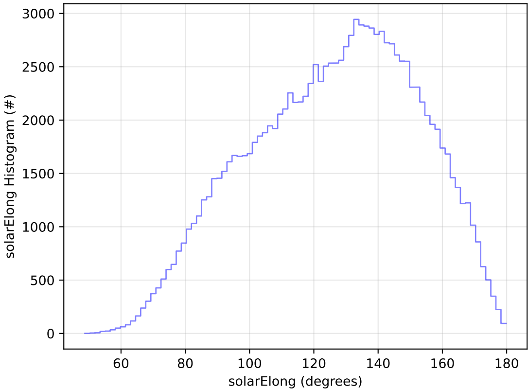
ddf_acor_sf25_lsf30_lsr10_v3.4_10yrs WFD u band: solarElong Histogram
