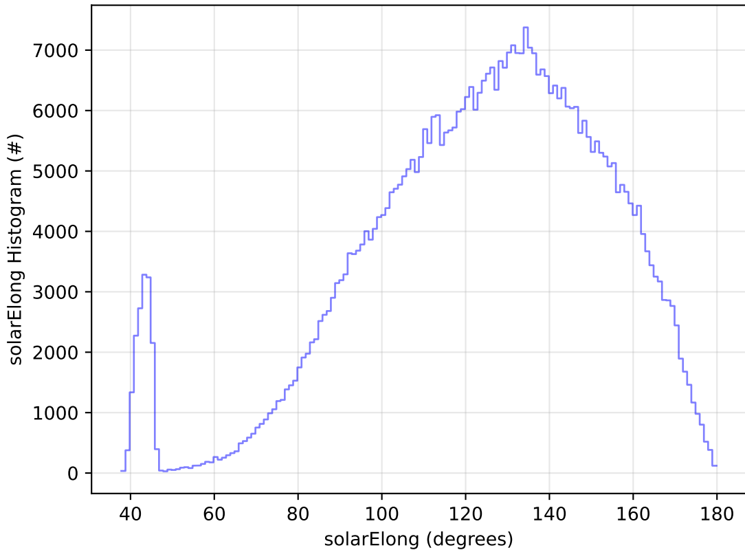
ddf_acor_sf25_lsf30_lsr10_v3.4_10yrs WFD r band: solarElong Histogram
