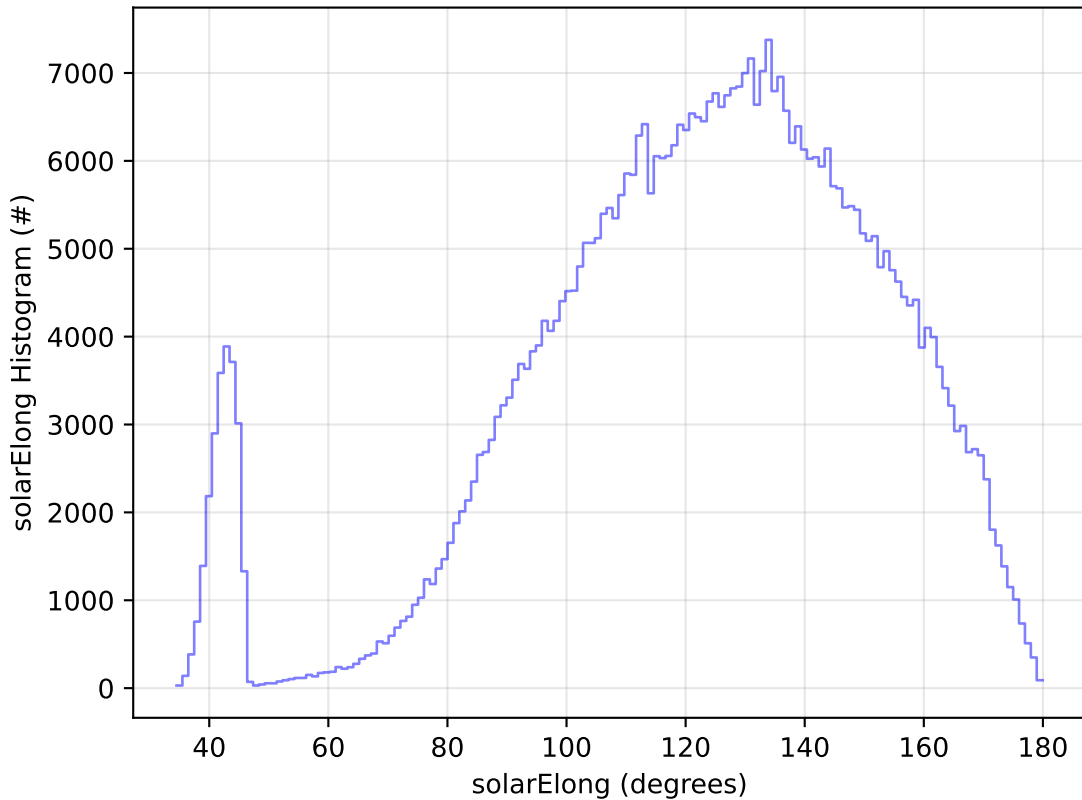
ddf_acor_sf25_lsf30_lsr10_v3.4_10yrs WFD i band: solarElong Histogram
