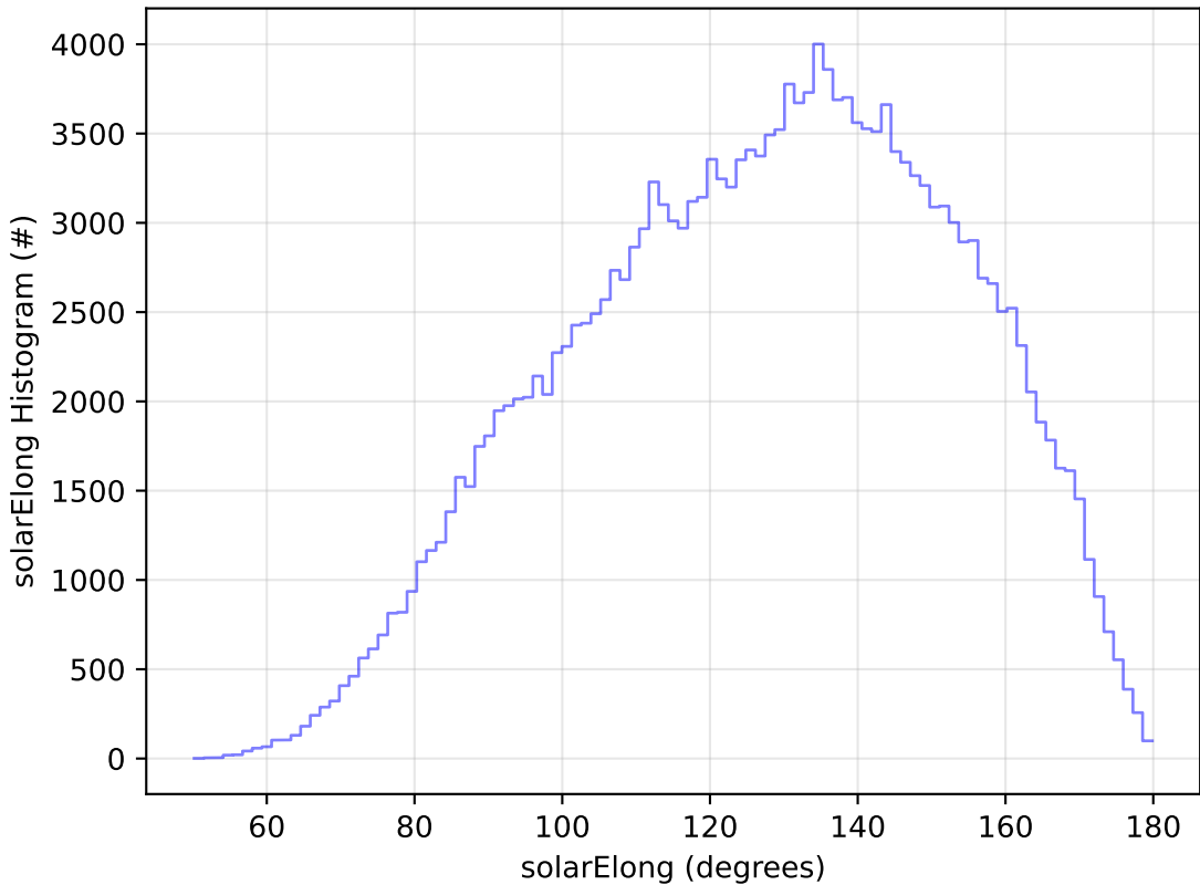
ddf_acor_sf25_lsf30_lsr10_v3.4_10yrs WFD g band: solarElong Histogram
