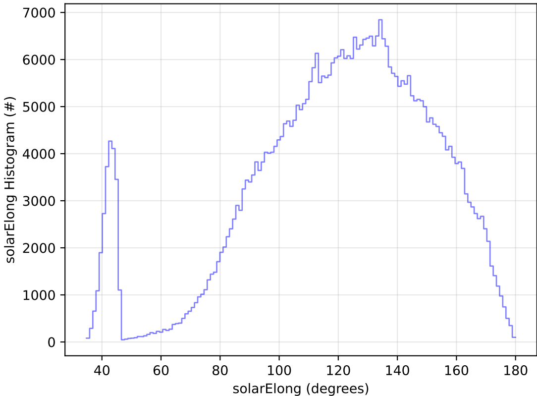
ddf_acor_sf25_lsf30_lsr10_v3.4_10yrs All sky z band: solarElong Histogram
