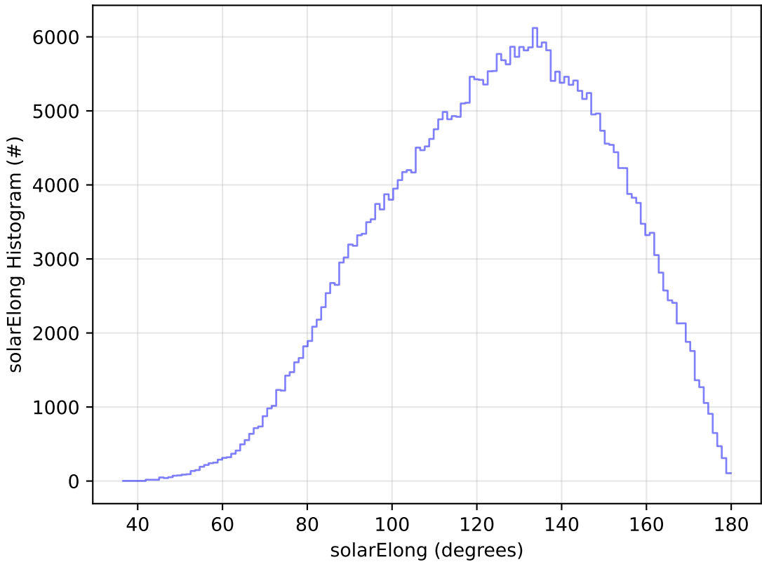
ddf_acor_sf25_lsf30_lsr10_v3.4_10yrs All sky y band: solarElong Histogram
