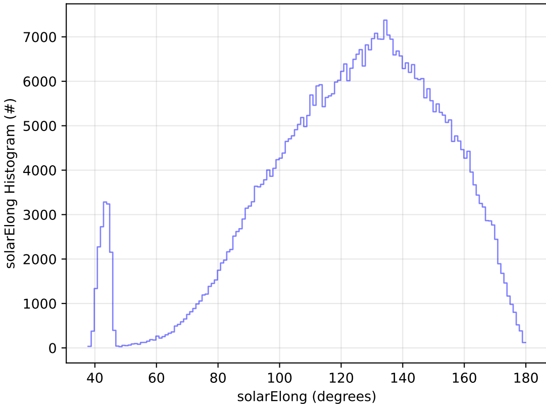
ddf_acor_sf25_lsf30_lsr10_v3.4_10yrs All sky r band: solarElong Histogram
