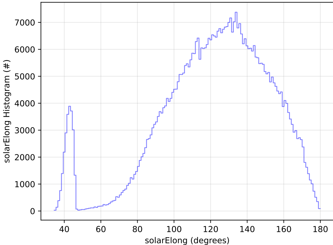
ddf_acor_sf25_lsf30_lsr10_v3.4_10yrs All sky i band: solarElong Histogram
