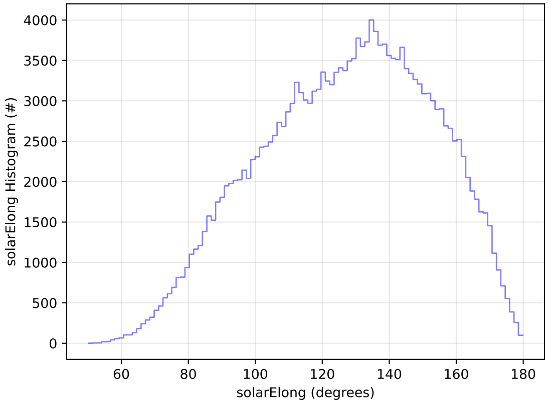
ddf_acor_sf25_lsf30_lsr10_v3.4_10yrs All sky g band: solarElong Histogram
