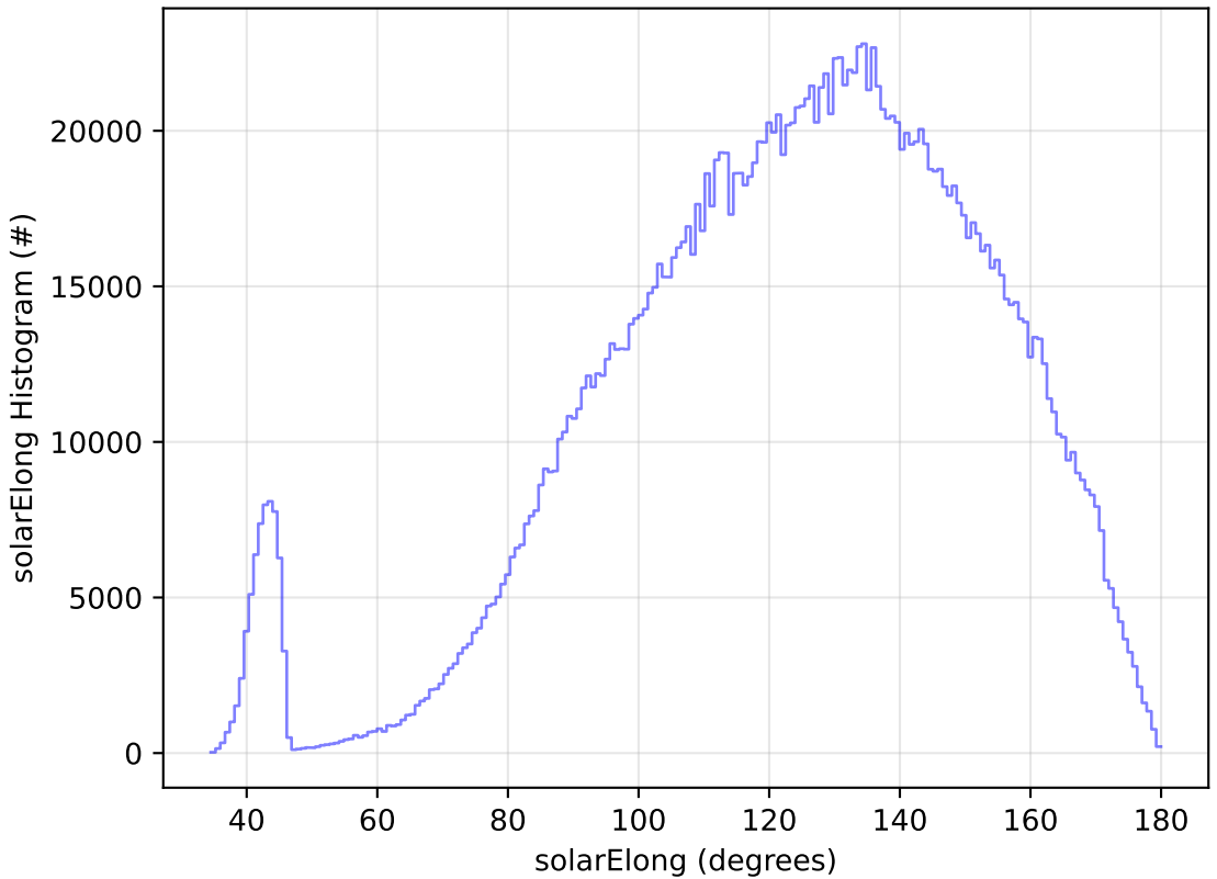
ddf_acor_sf25_lsf30_lsr10_v3.4_10yrs All sky all bands: solarElong Histogram
