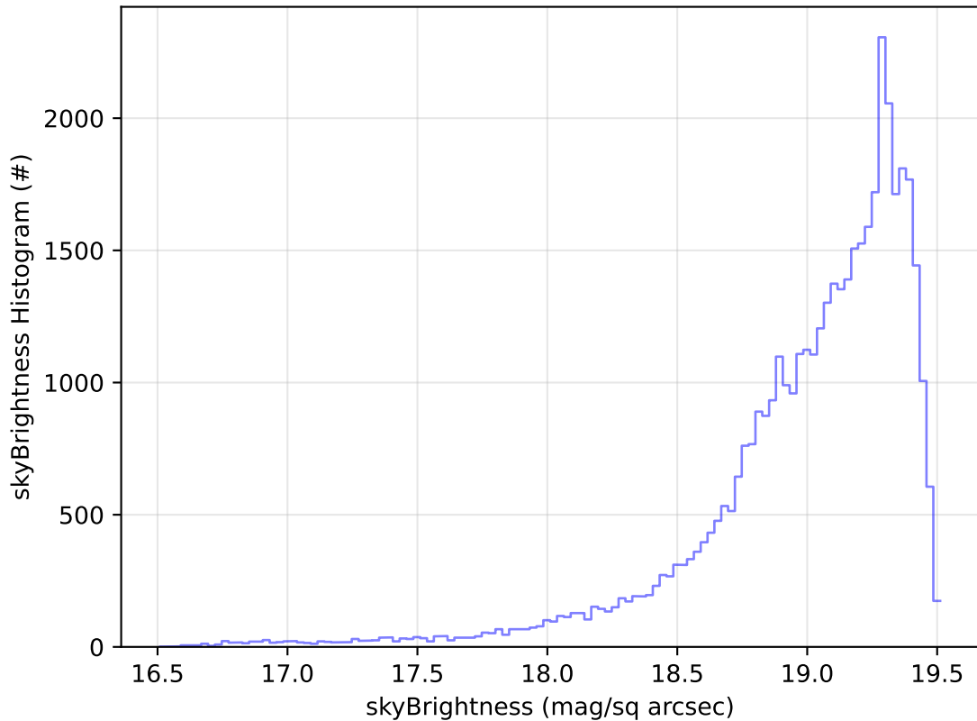
ddf_acor_sf25_lsf30_lsr10_v3.4_10yrs Yr 1 z band: skyBrightness Histogram
