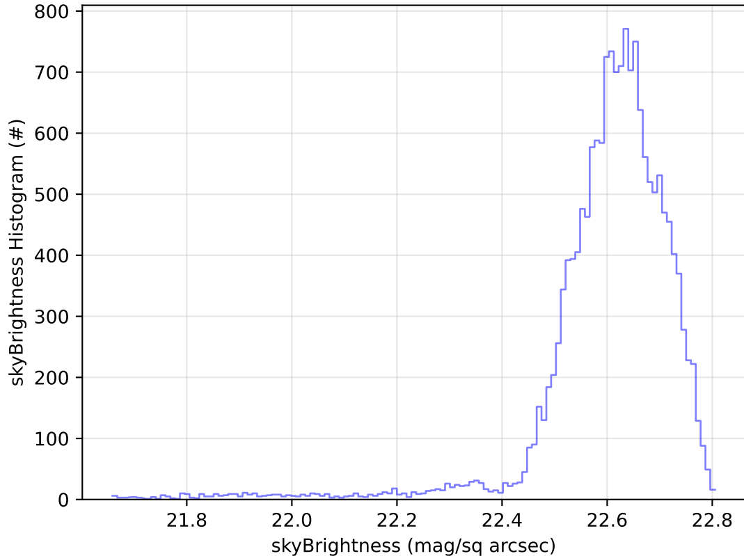
ddf_acor_sf25_lsf30_lsr10_v3.4_10yrs Yr 1 u band: skyBrightness Histogram
