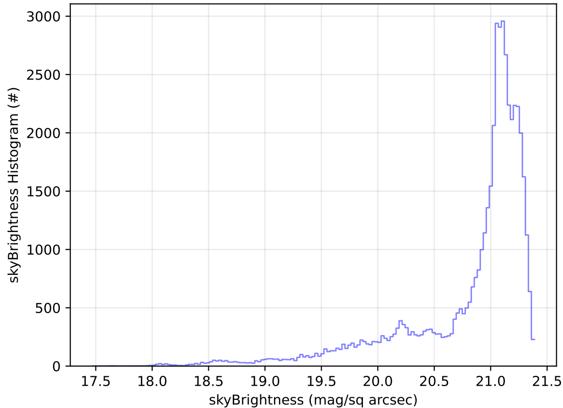
ddf_acor_sf25_lsf30_lsr10_v3.4_10yrs Yr 1 r band: skyBrightness Histogram
