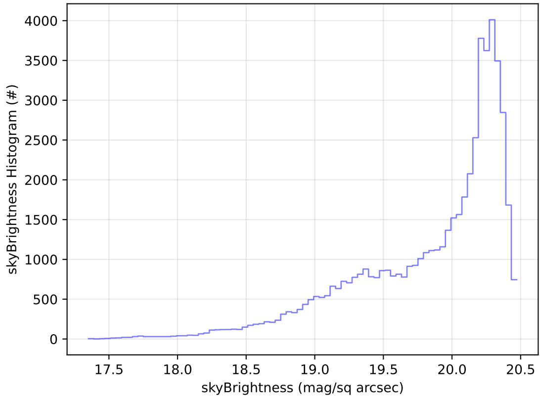
ddf_acor_sf25_lsf30_lsr10_v3.4_10yrs Yr 1 i band: skyBrightness Histogram
