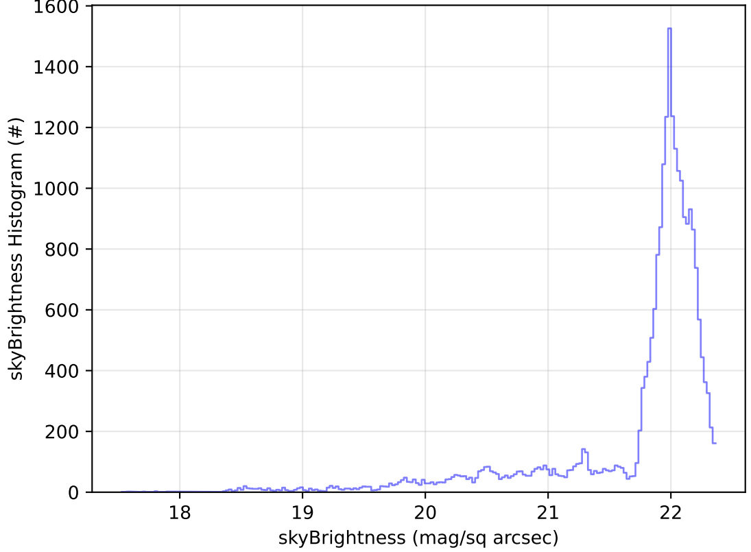
ddf_acor_sf25_lsf30_lsr10_v3.4_10yrs Yr 1 g band: skyBrightness Histogram
