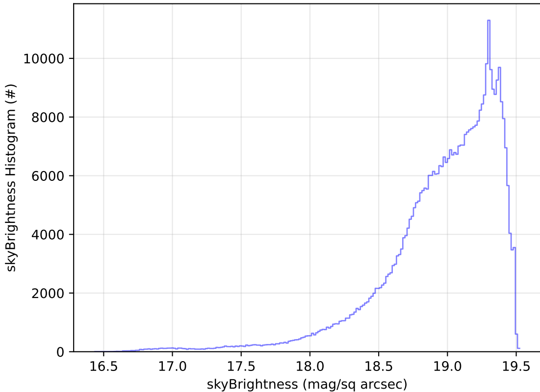
ddf_acor_sf25_lsf30_lsr10_v3.4_10yrs WFD z band: skyBrightness Histogram
