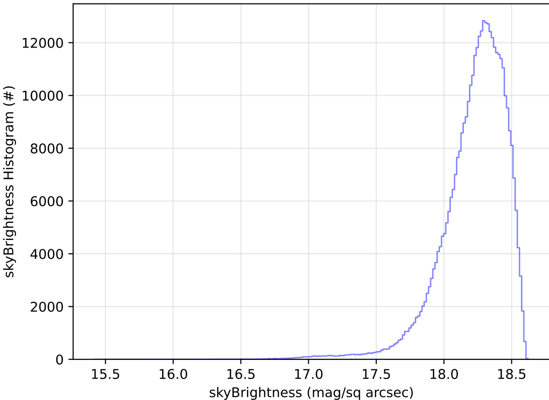
ddf_acor_sf25_lsf30_lsr10_v3.4_10yrs WFD y band: skyBrightness Histogram
